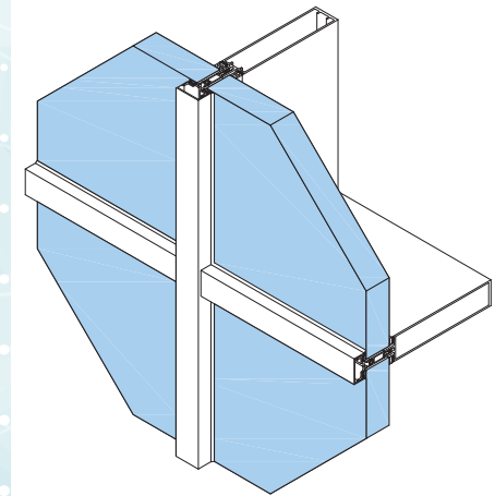
CURTAIN WALL SYSTEM - CW35
