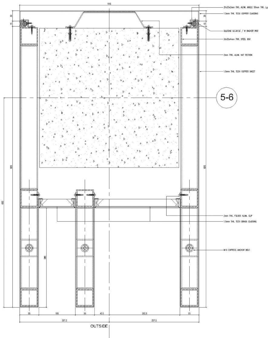
COLUMN CLADDING WITH TECU COPPER
