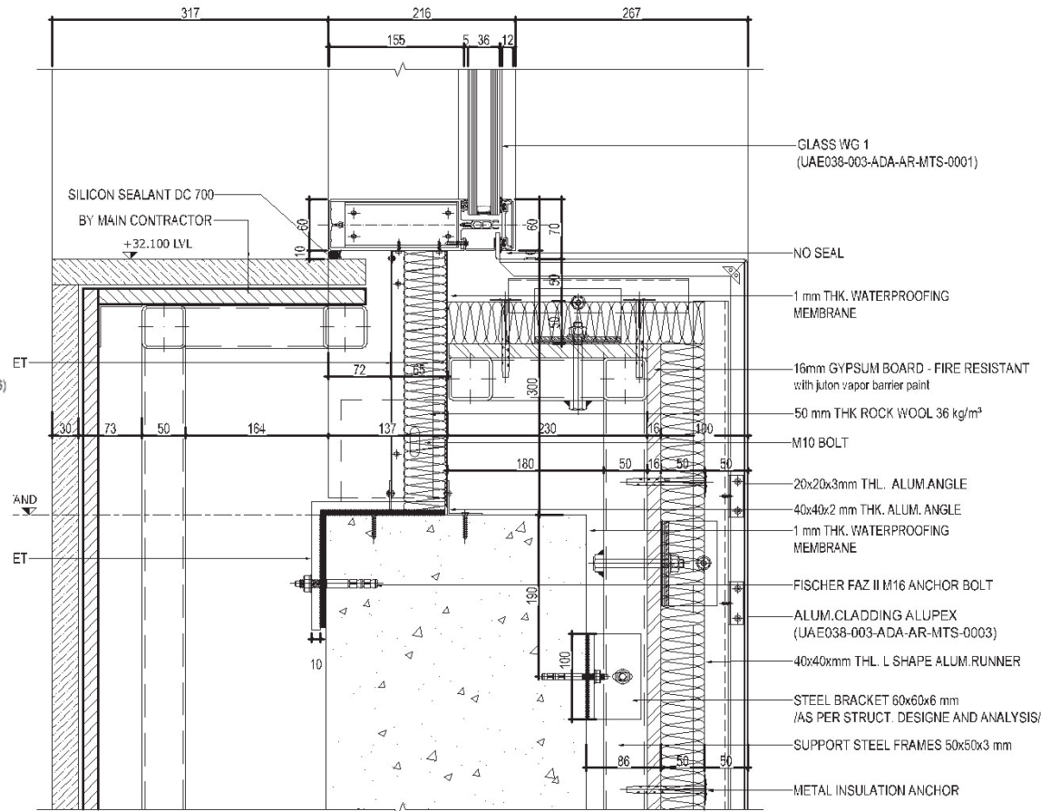
TRANSOM SILL DETAIL
