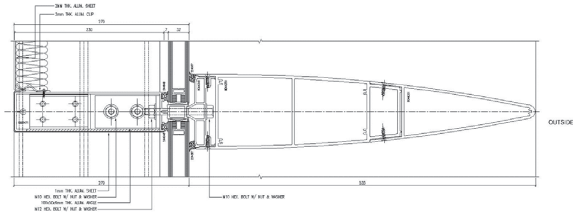
TRANSOM INT. DETAIL
