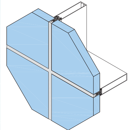
CURTAIN WALL SYSTEM - CW35 | SG
