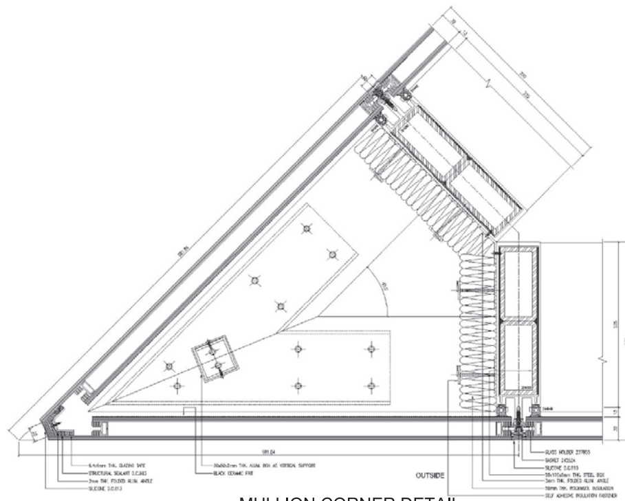
MULLION CORNER DETAIL
