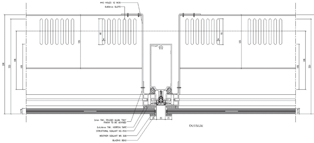
MULLION INT. DETAIL
