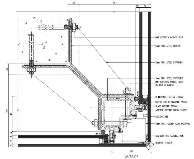
CORNER DETAIL
