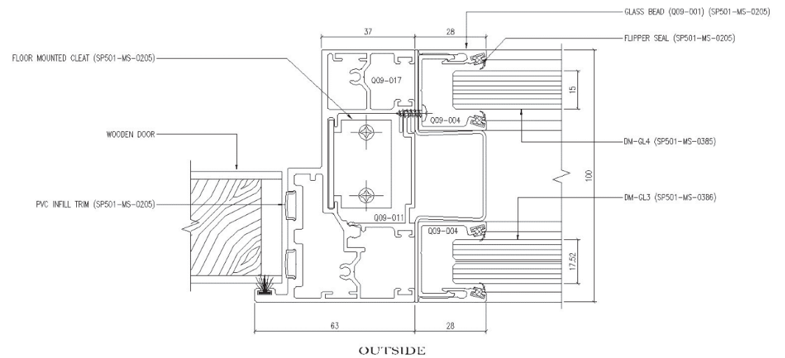
DEMOUNTABLE PARTITION DOOR JAMB DETAIL
