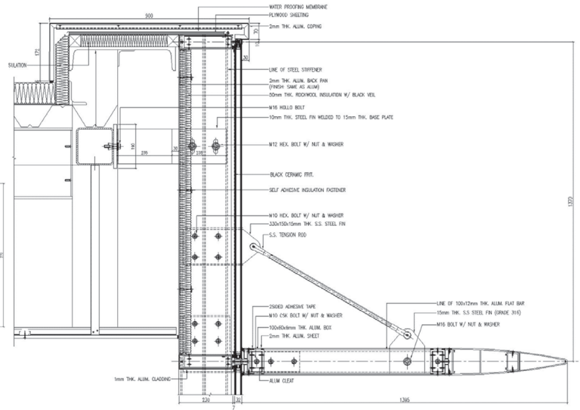
TRANSOM WITH SUNSHADE DETAIL
