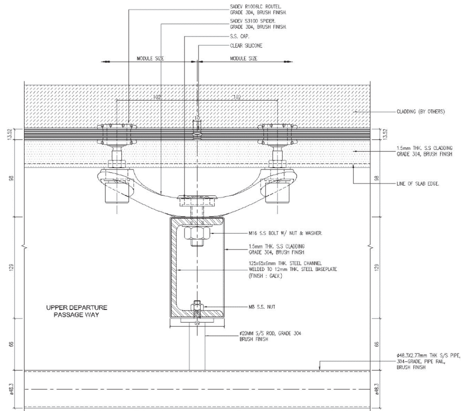
POINT FIXED INTERMEDIATE DETAIL
