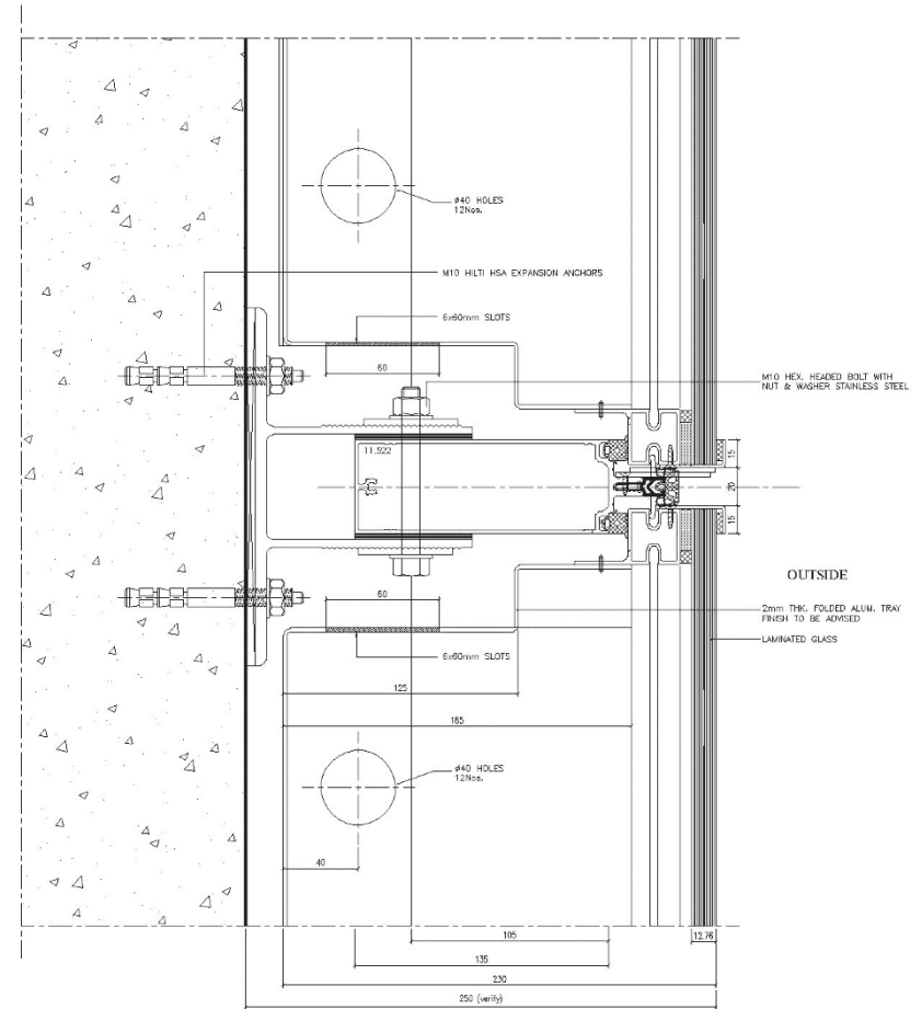
TRANSOM INT. DETAIL
