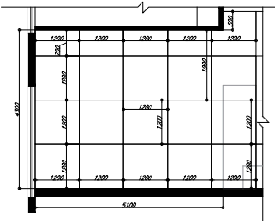
2 DXB ISLAND - LIVING AREA FLOOR - AREA (A) SCALE 1:50 METERS
