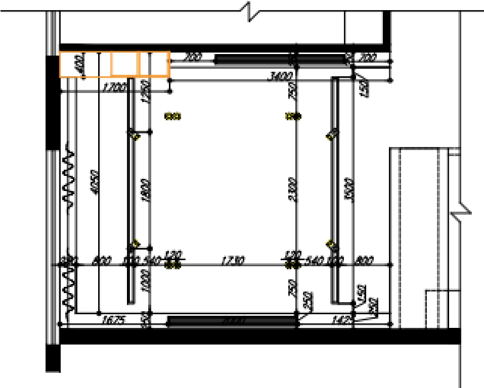
3 DXB ISLAND - LIVING AREA CEILING - AREA (A) SCALE 1:50 METERS
